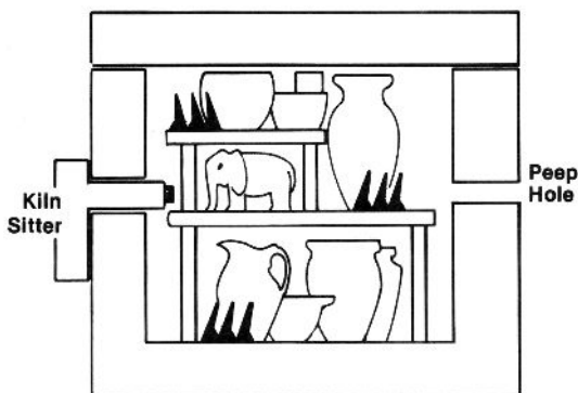
Sectional view of kiln chamber showing Self-Supporting Cones in several locations.
