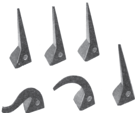
Self-Supporting Cones before and after firing.
